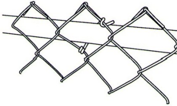
Tie Wire Detail
