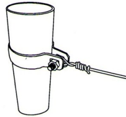
Tension Wire Detail
