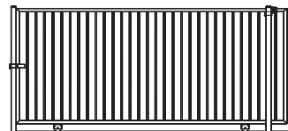
V-TRACK ROLL GATES Standard up to 40' opg x 10' height
