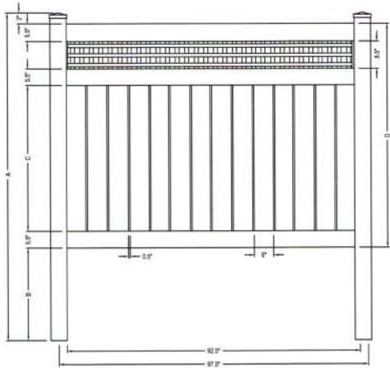
FRONT ELEVATION
