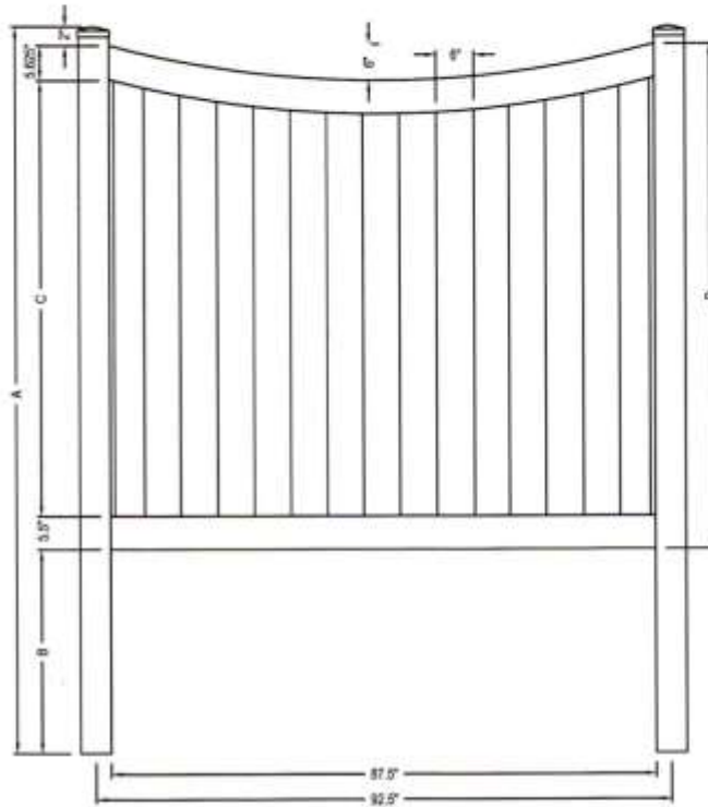
FRONT ELEVATION
