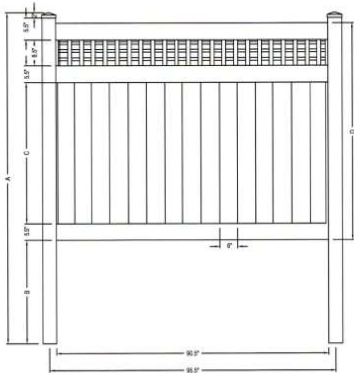
FRONT ELEVATION
