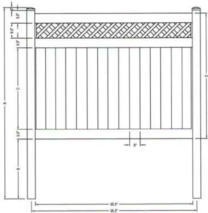
FRONT ELEVATION
