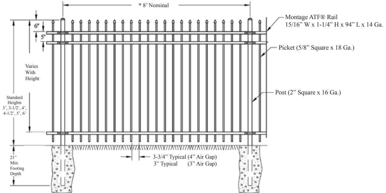
TYPICAL PANEL DRAWING (Classic Style shown; Genesis, Majestic, Warrior, Crescent and Gemini also available)
