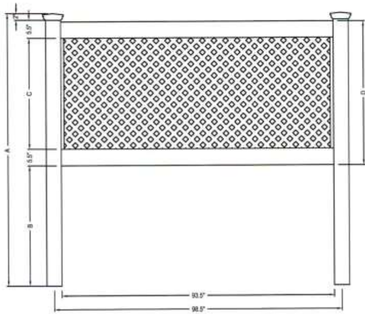
FRONT ELEVATION
